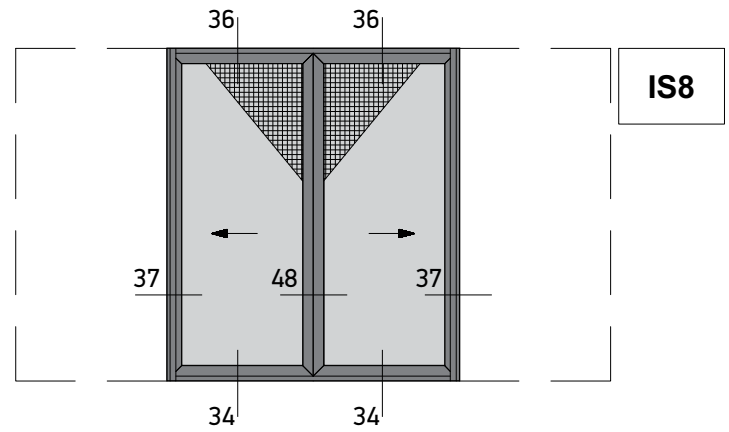
Pocket Sliding Window with Meeting Stile and Narrow Flyscreen
