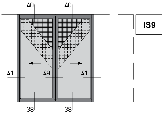
Pocket Sliding Window with Meeting Stile, with Flyscreen and Shutter
