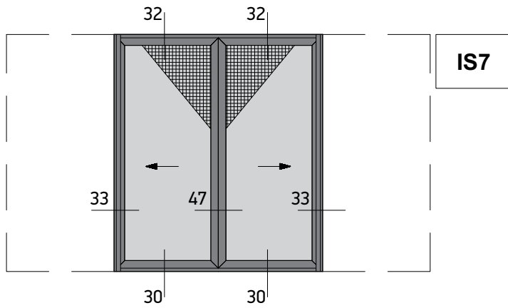
Pocket Sliding Window with Meeting Stile and Flyscreen
