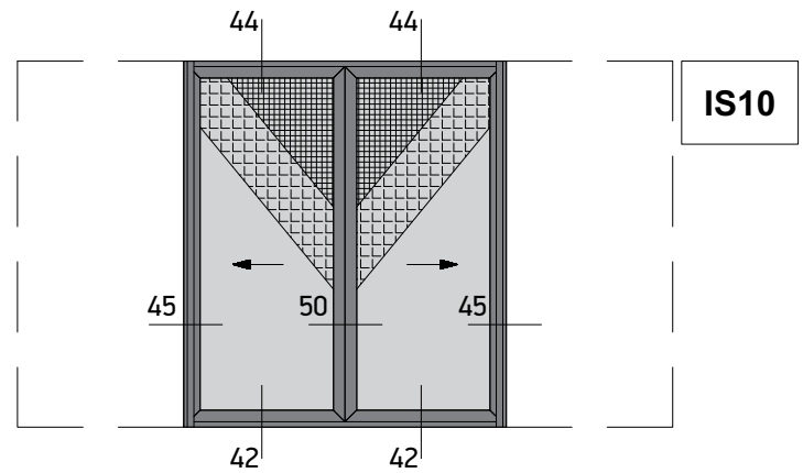
Pocket Sliding Window with Meeting Stile, with Narrow Flyscreen and Shutter
